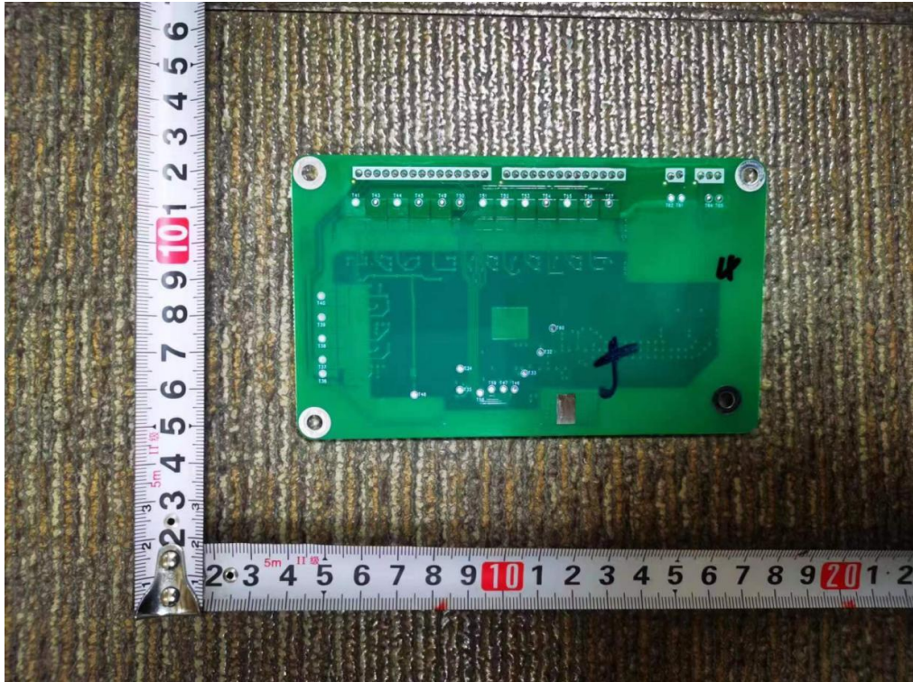
Slave control board in Battery module (Bottom view)
