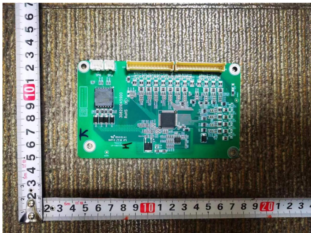
Slave control board in Battery module (Top view)
