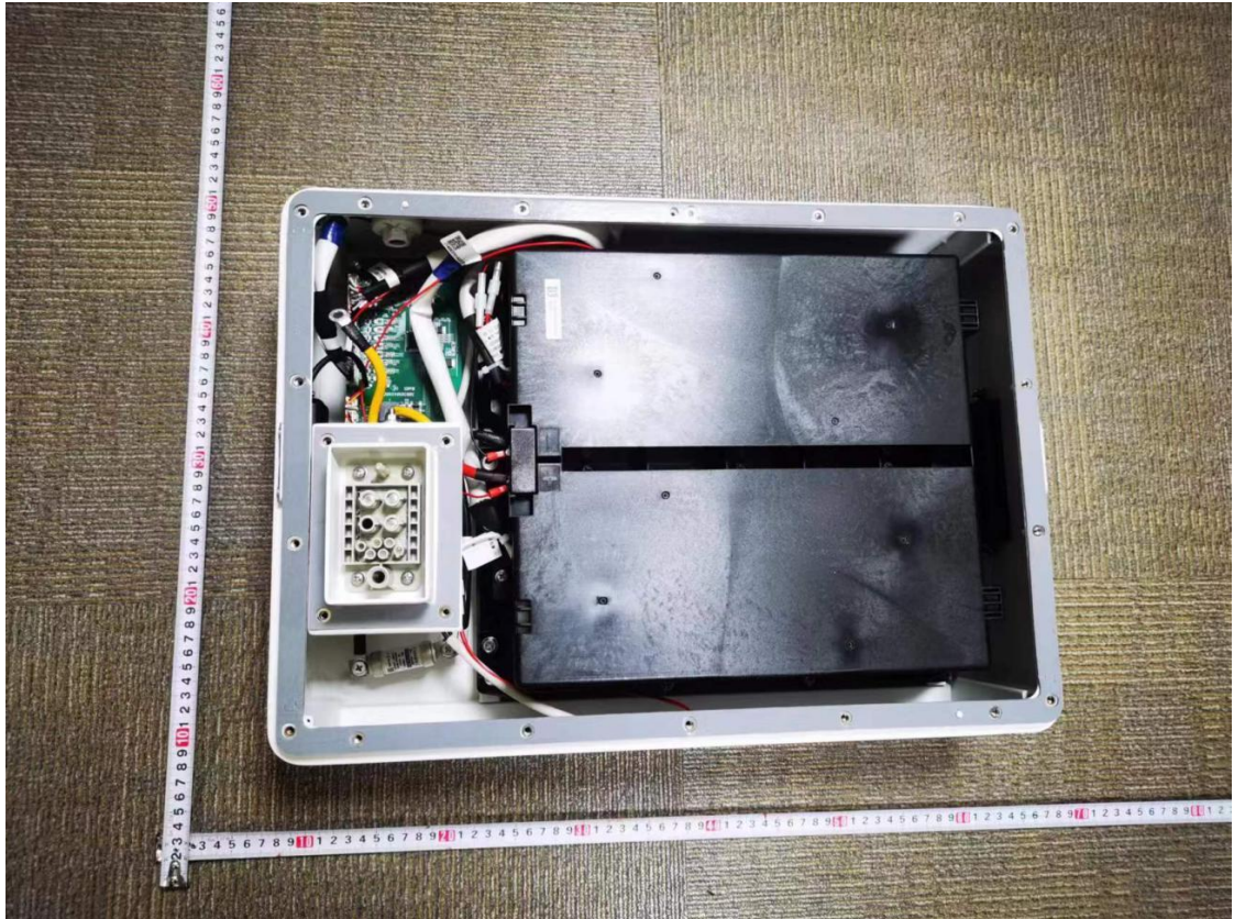
Battery module, Model: TP-HS25, (Insided view)
