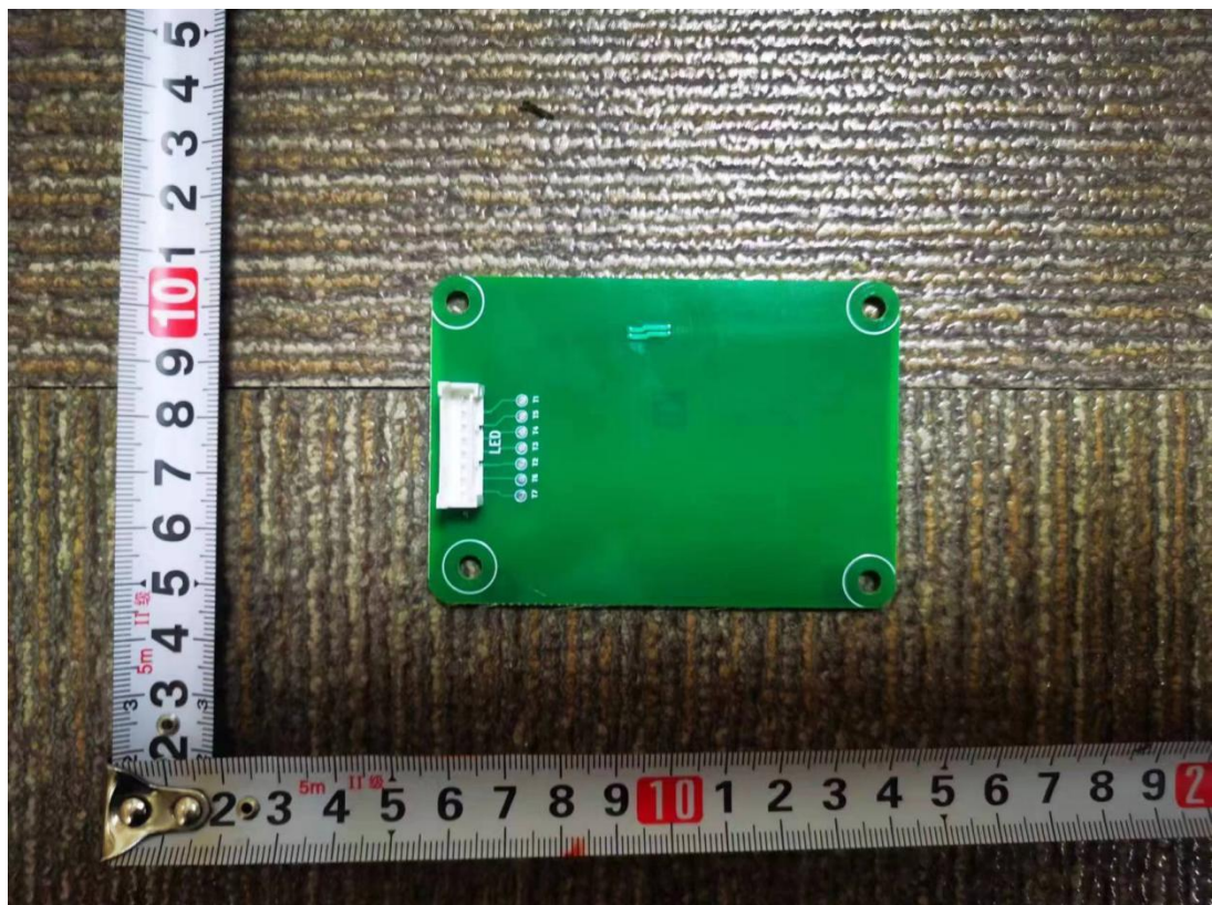
Light board in Main control unit (Bottom view)
