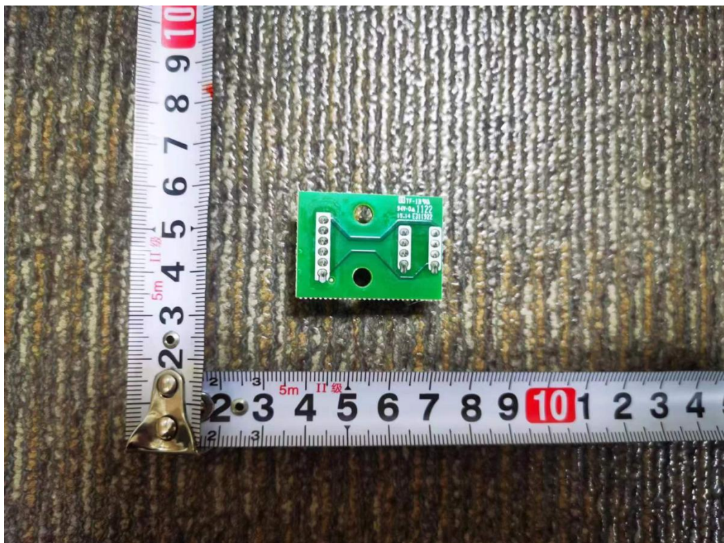
Dip switch board (Bottom view)
