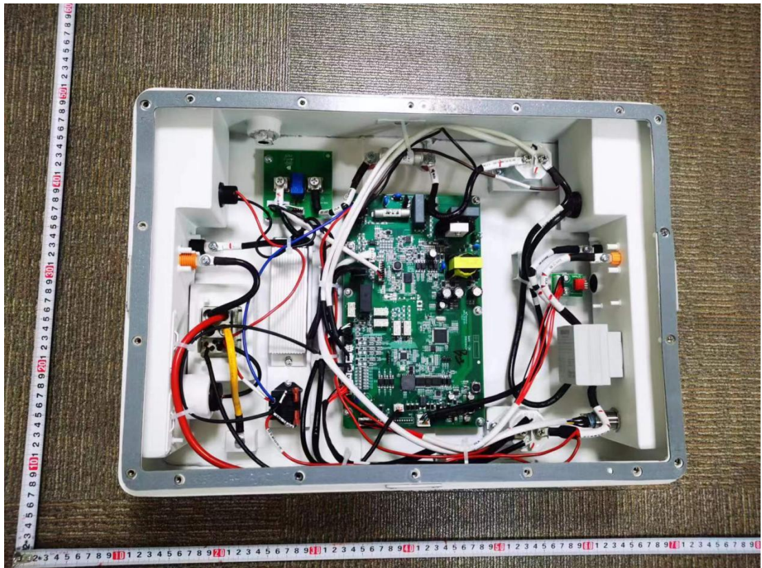
Inside of Main control unit, Model: TBMS-MCS0800
