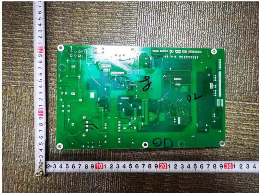
Main control board in Main control unit (Bottom view)
